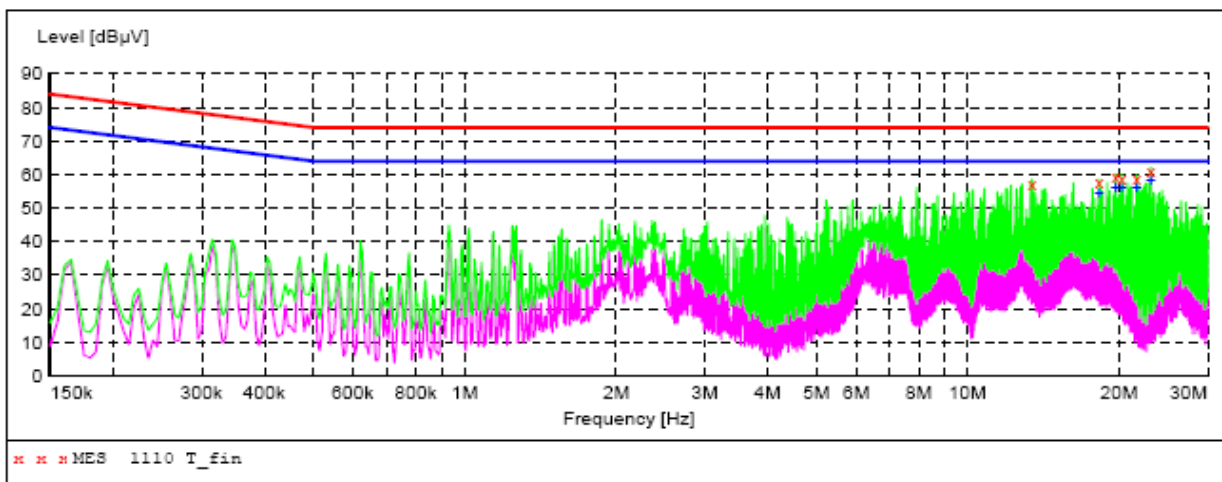
SCAN TABLE: "Voltage(150K-30M)FIN" Short Description: 150K-30M Voltage
