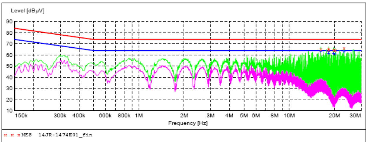
SCAN TABLE: "Voltage (150K-30M) FIN" Short Description: 150K-30M Voltage
