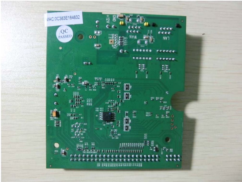
MAIN PCB2
