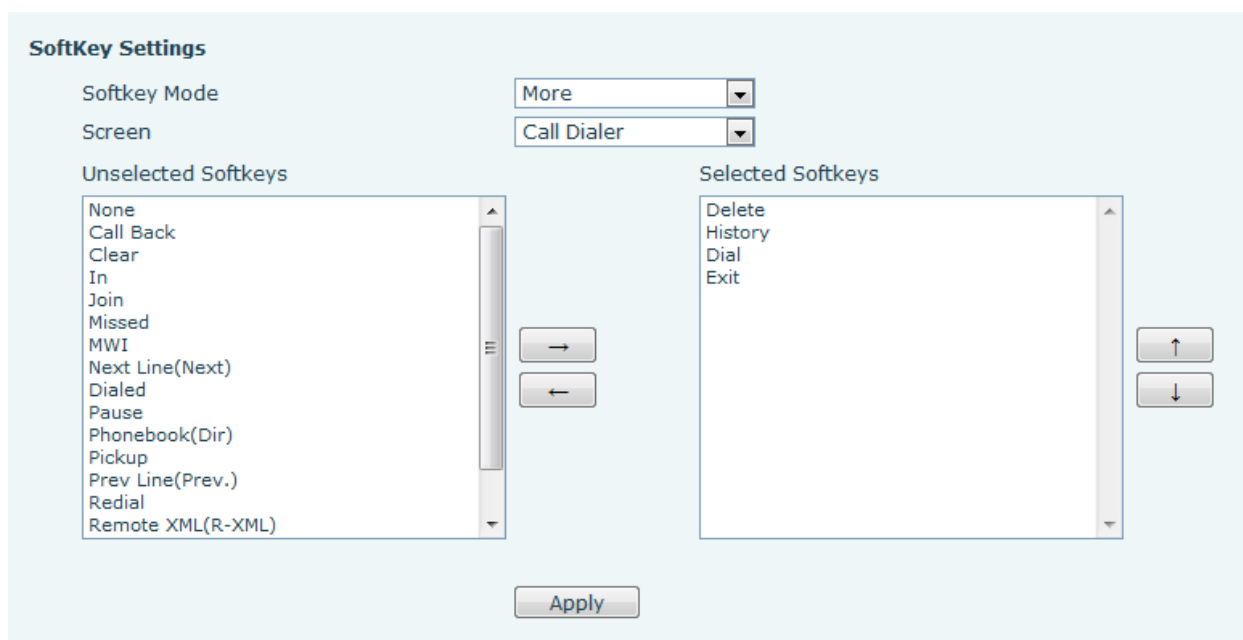
Figure 58 – Softkey Configuration
